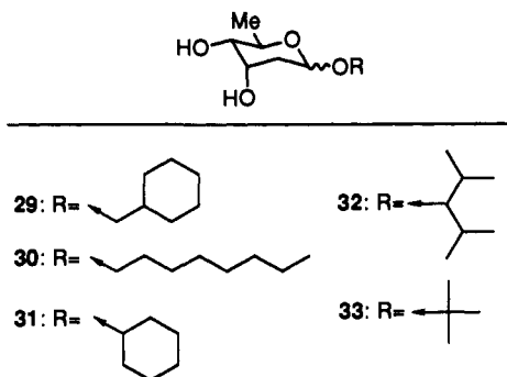
Figure 6. 2,6-Dideoxy glycosides.
